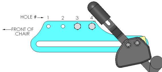
Down-Rearward, Holes 3&4
