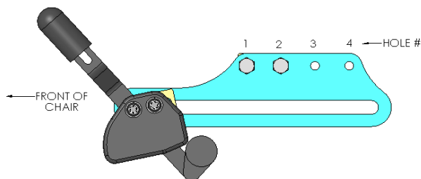
Down-Forward, Holes 1&2
