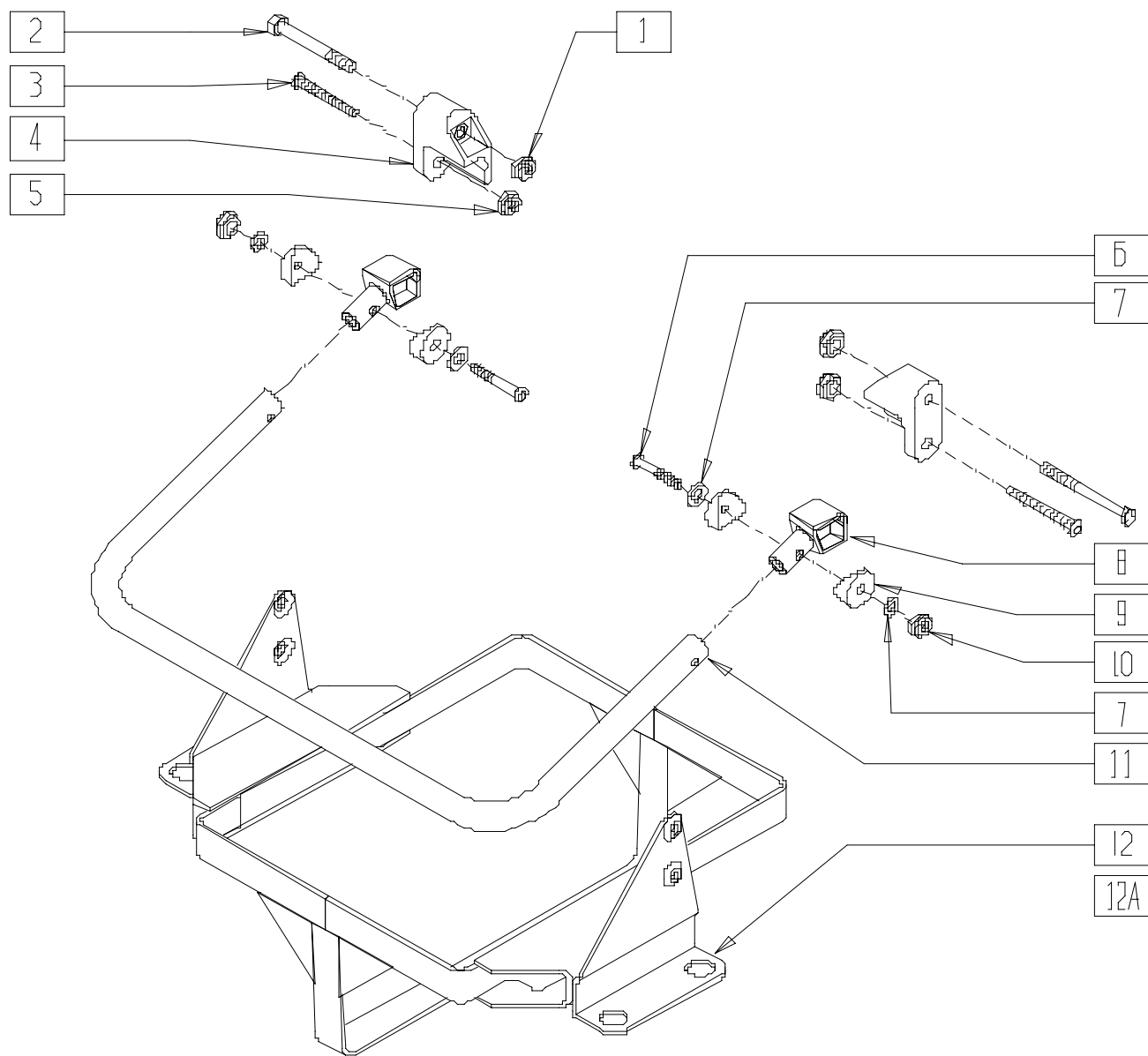
Drawing shows 20" Battery Cage. 14" - 18" Cages are slightly different.
