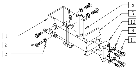
QUICKIE Z500(ZIPPIE P500) RECEIVER ASSEMBLY: 880244 (INCLUDES ITEMS: 1 3,5,15 17)
