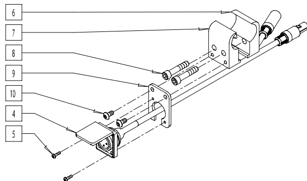
QUICKIE Z500 TILT
